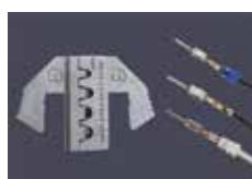
DSQIL1 For VAG male terminals 0,5-2,5 mm 2 with and without seal
