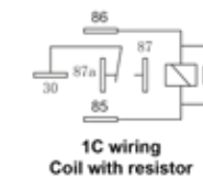
RE62024CBR Miniature relay with insulating mounting bracket 24V, 20/15A, 1,6W 26,5 x 26,5 x 24,5 (+16) mm
