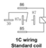
RE620Q24C Miniature relay 24V, 40/30A, 1,6W 35,5 x 35,5 x 45 mm Waterproof in combination with SOCKET04 and SOCKET04-5
