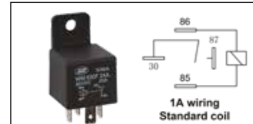
RE630FA24B Miniature relay with insulating mounting bracket 24V, 20A, 1,6W 28 x 28 x 25,5 (+16) mm
