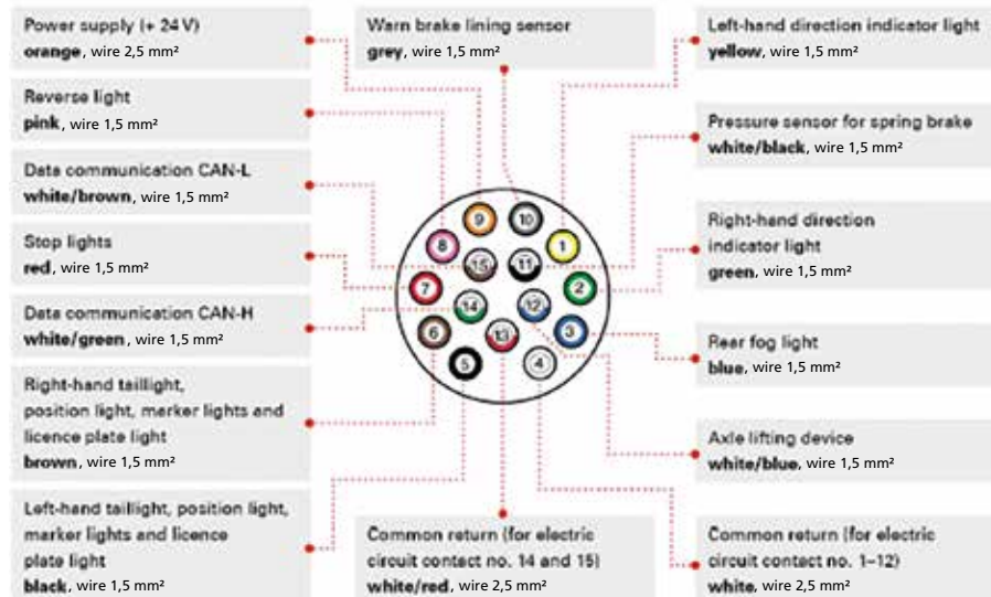
24SC003 15 pole Screw contacts
