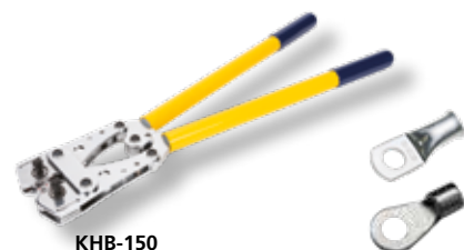
KHB-150 26" Crimping tool for non-insulated terminals 25,0 - 150,0 mm 2 HEXAGONAL crimp
