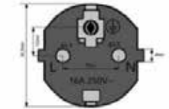
CEE7/7 Plug (French-Schuko standard)
